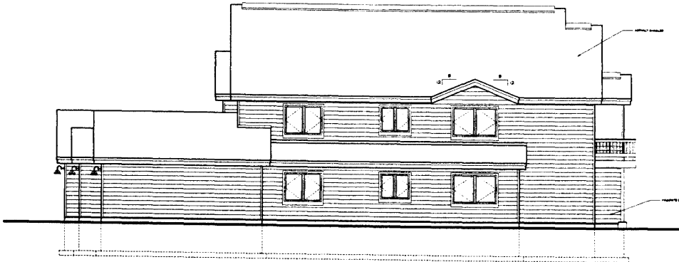
SIDE ELEVATION SCALE 1/4" = 1'-0"
